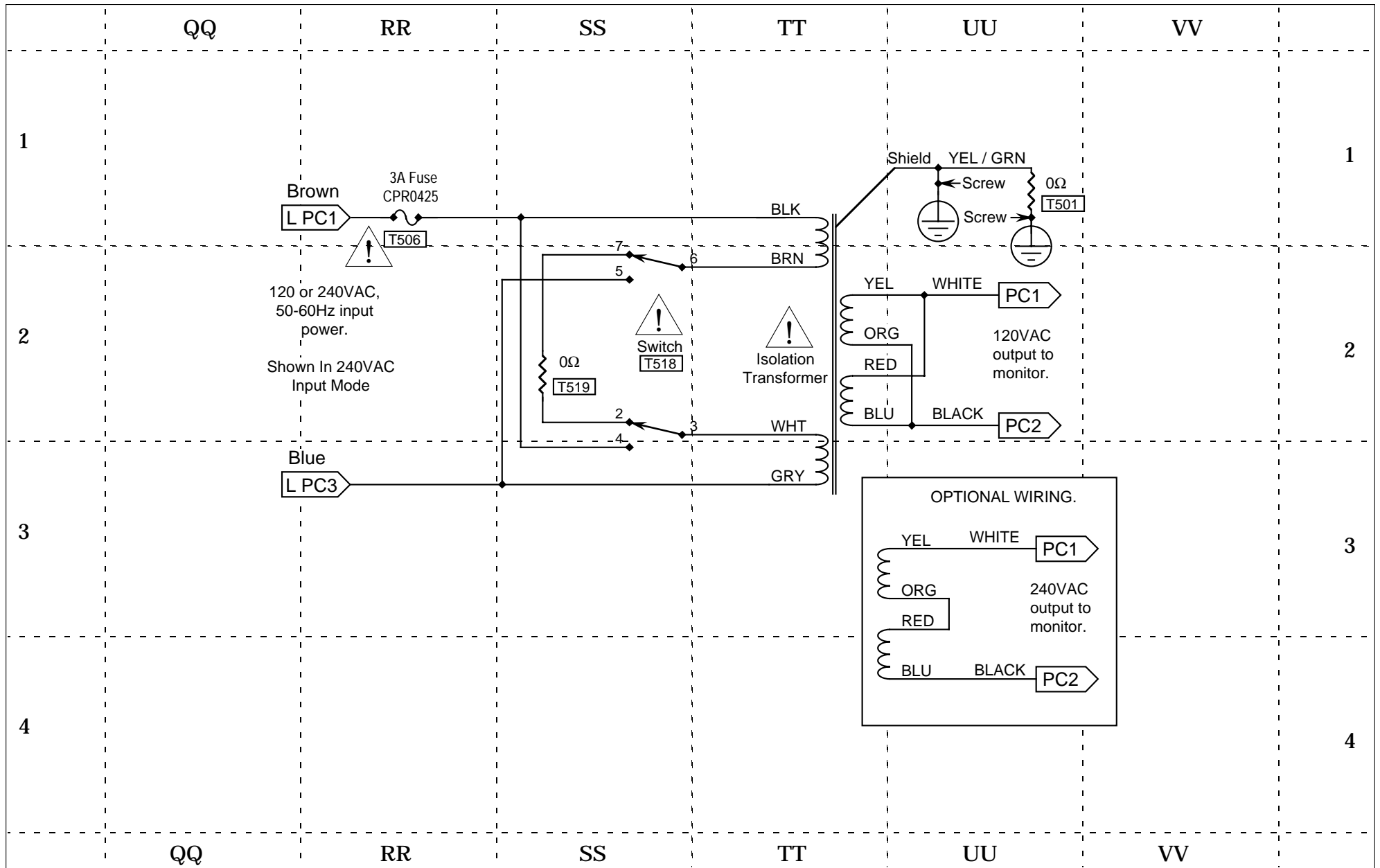
CERONIX CPA4159 SCHEMATIC Model ISO XFR-75W, MANUAL Date; 06/12/02
