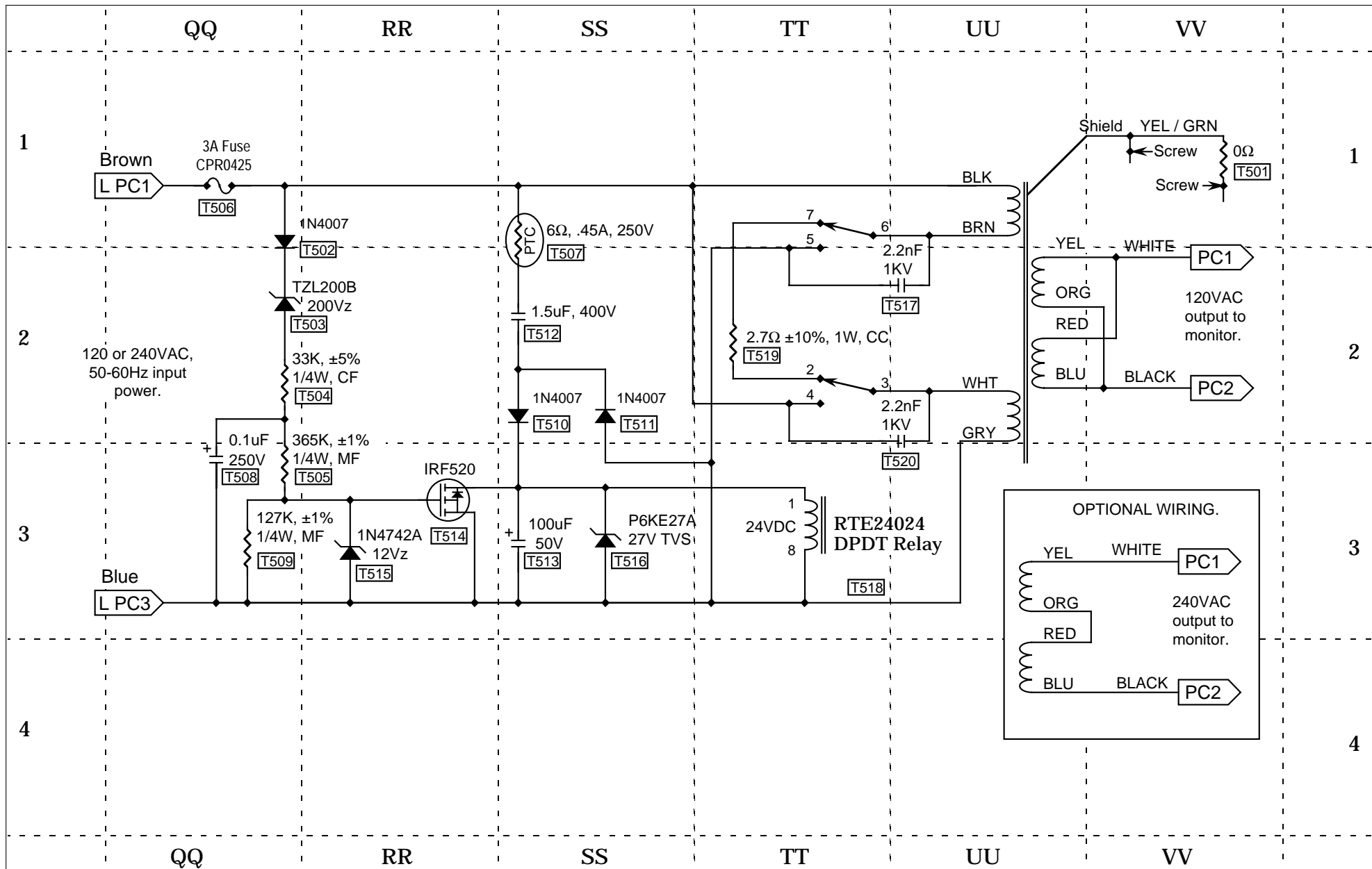
CERONIX CPA4147 SCHEMATIC Model ISO XFR-75W, AUTO Date; 06/12/02
